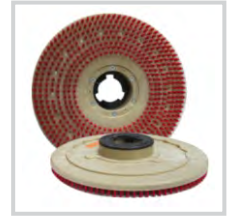
Tufted Pad Driver w/ Riser Molded Plastic Block, 1" Riser #A0010-4 - 17" #A0011-3 - 20"
